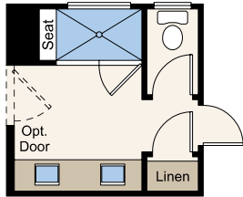
OPT. SHOWER WITH SEAT AT PRIMARY BATH
