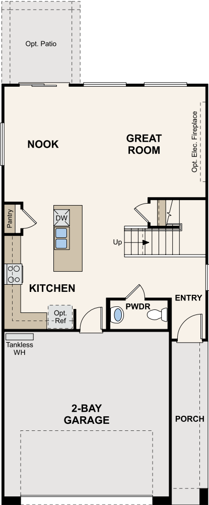
MAIN LEVEL
